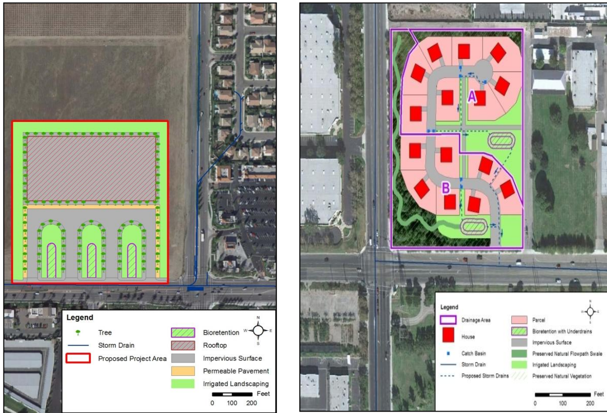
Figure 5-3. WQMP Site Design for Commercial and Residential Case Studies
